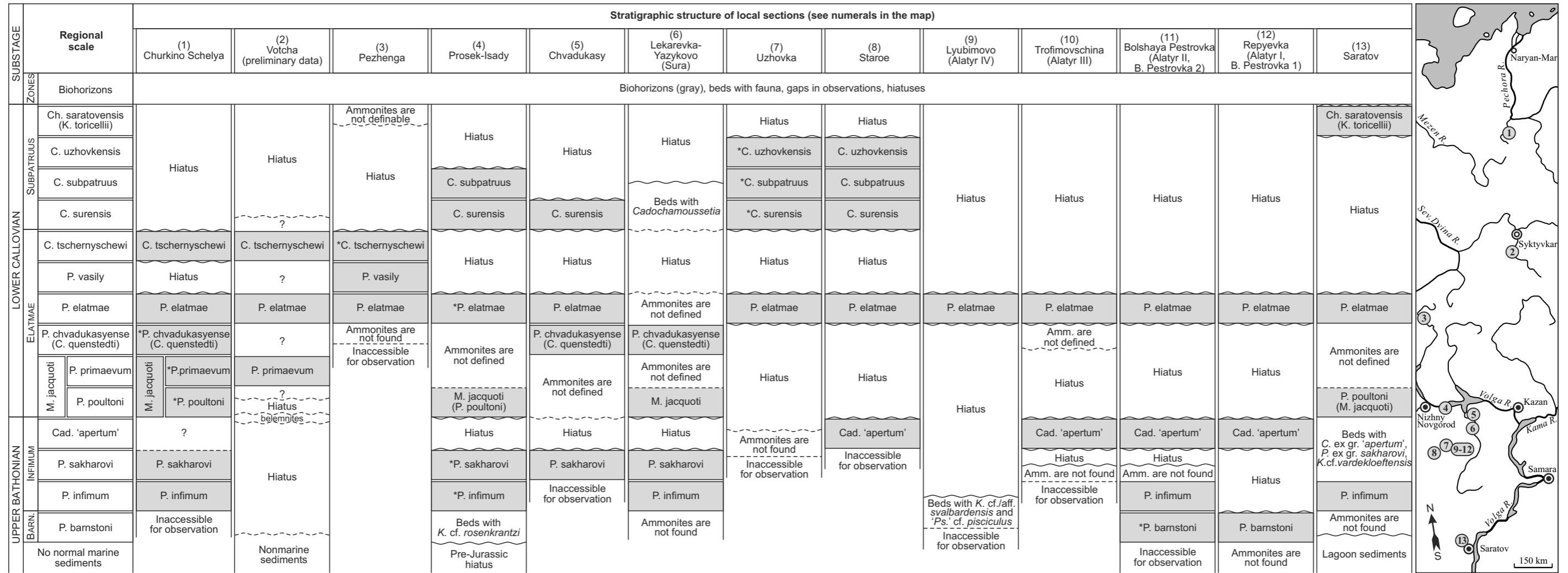
Fig. 2. Correlation of local sections of Bathonian-Callovian boundary interval of European Russia (D.B. Gulyaev, 2015 - under construction)
